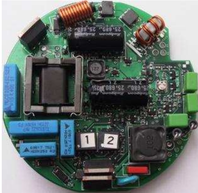
21W ballast to drive miniature HID xenon bulbs with AC current powered by Nucon®
